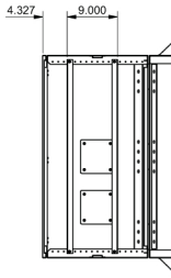
SECTION A-A (RIGHT SIDE VIEW)
