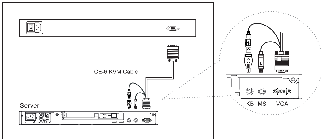
Figure 6. Example of connecting CE-6 4-in-1 Combo KVM cable to server via PS/2 interface
