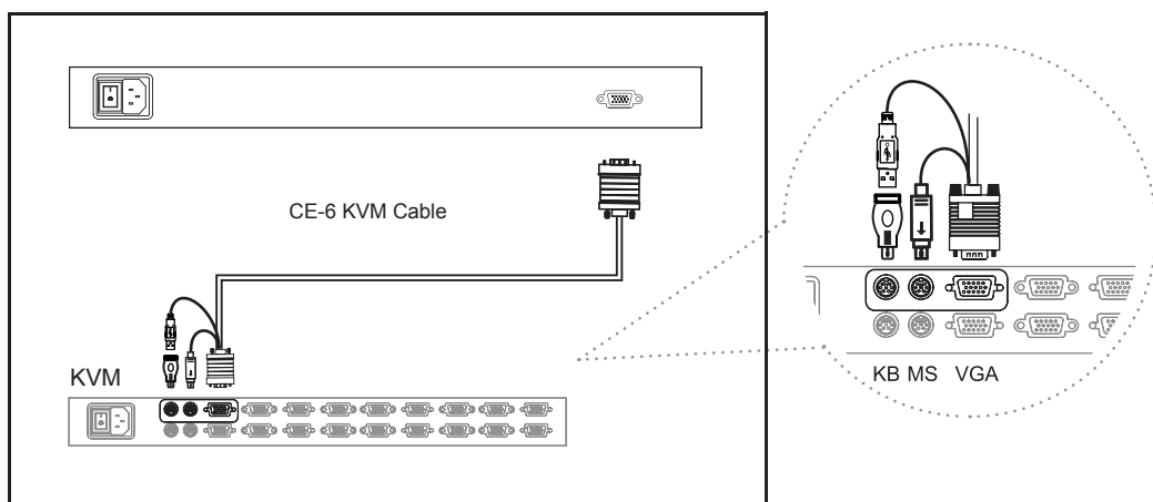
Figure 7. Example of connecting CE-6 4-in-1 Combo KVM cable to KVM via PS/2 interface
