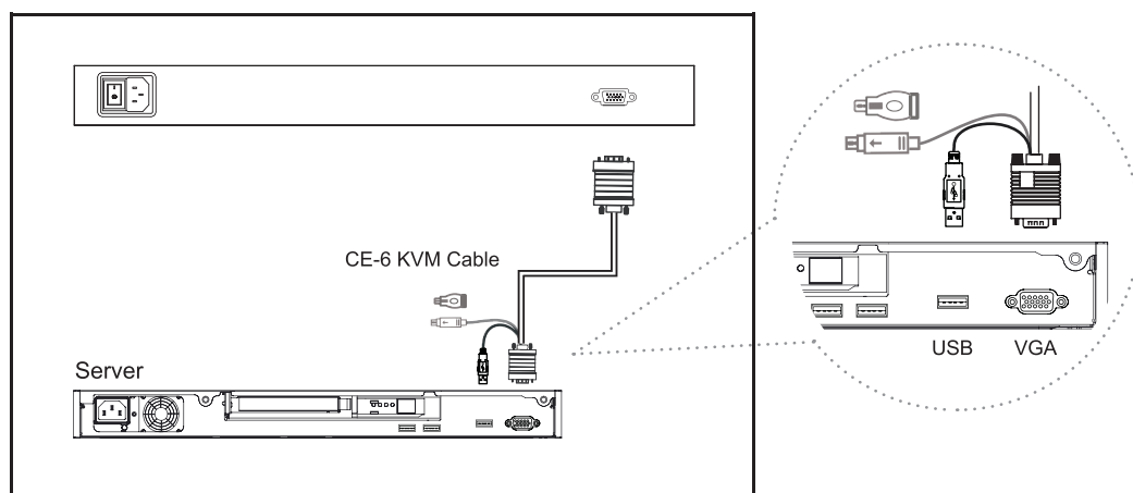
Figure 8. Example of connecting CE-6 4-in-1 Combo KVM cable to server via USB interface
